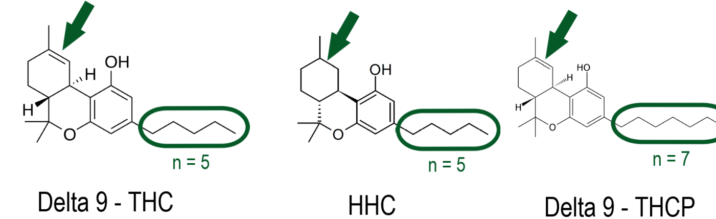
Figure 2: Chemical Structures of d9-THC vs HHC vs d9-THCP
