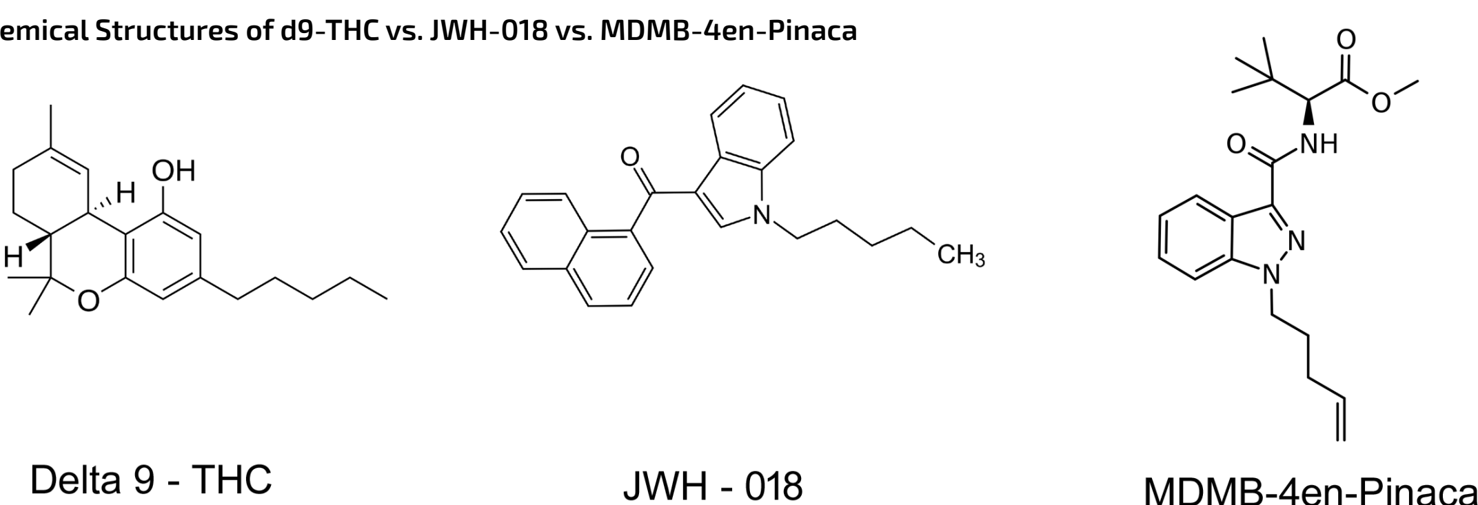
Figure 3: Chemical Structures of d9-THC vs. JWH-018 vs. MDMB-4en-Pinaca
